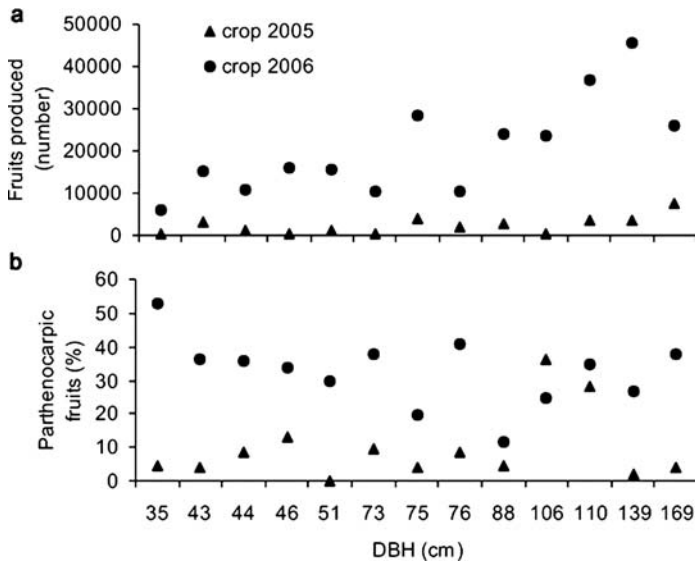
Fig. 11.2 Number of fruits (a) and percentage of parthenocarpic fruits (b) produced by 13 trees of Bursera morelensis during the years 2005 and 2006 in the Tehuacan Valley, México. Trees are arranged in accordance with diameter at breast height (DBH)
