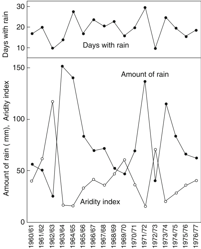
Fig. 21.2 Number of rainy days, annual precipitation and aridity index as given by the ratio of evaporation and precipitation in the Negev desert in the years 1960–1977
